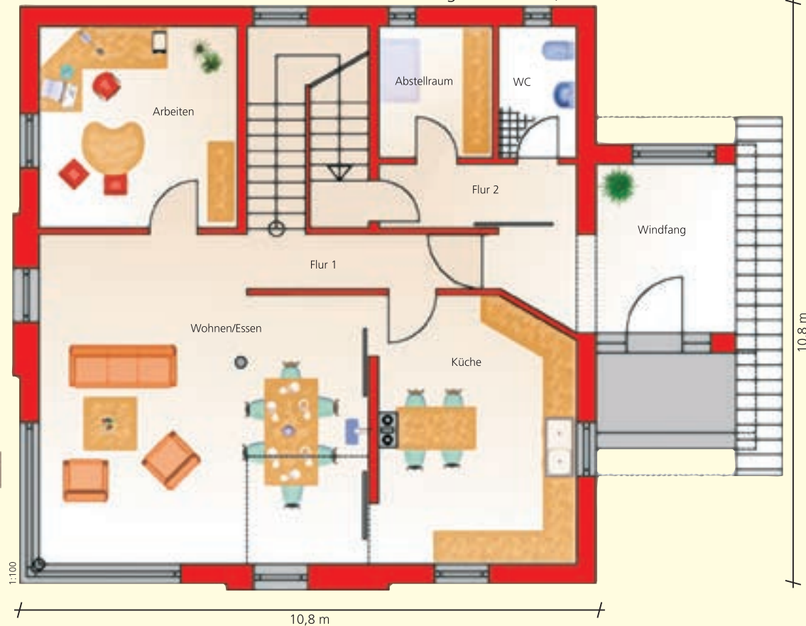
Erdgeschoss* 96,0 m 2
